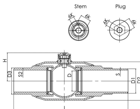
DN 20 - 40
